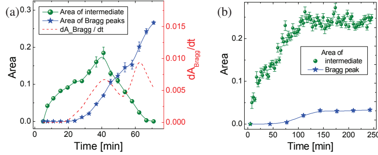
Figure 8 Time-dependence of the area of the broad peak ( A_{\text{intermediate}} ) and the Bragg peaks ( A_{\text{Bragg}} ). Green spheres (left axis) show A_{\text{intermediate}}(t) , the integral of the broad Gaussian function connected to the intermediate. Blue stars (left axis) show A_{\text{Bragg}}(t) , the integral of the two Bragg peaks in this area. (a) BLG 33 mg/ml with 17 mM \text{CdCl}_2 . For clarity and better statistics, always three data points of A_{\text{intermediate}}(t) and A_{\text{Bragg}}(t) were merged into one. The dashed red line in corresponds to the first derivative of the area of Bragg peaks as a function of time (right axis). (b) BLG 33 mg/ml with 20 mM \text{CdCl}_2 .
