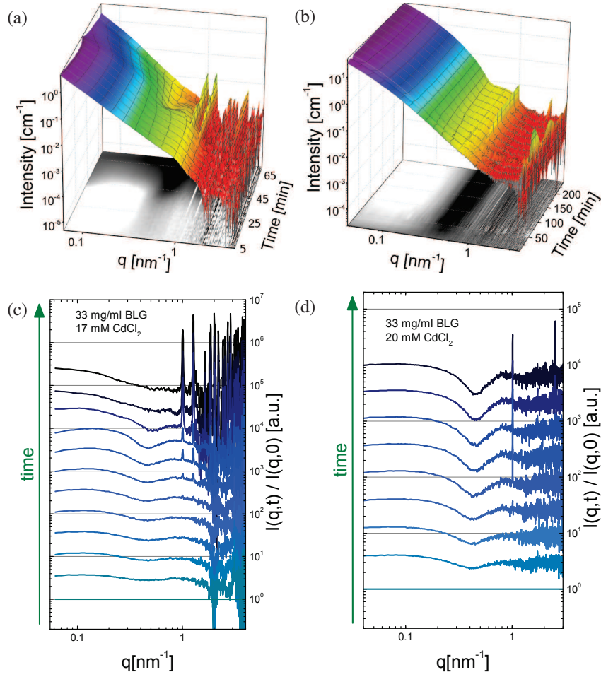
Figure 7 Protein crystallization followed by real-time SAXS measurements. Samples contain 33 mg/ml BLG with 17 mM CdCl 2 (a&c) and 20 mM CdCl 2 (b&d), located in the transition zone of pseudo-c** (i.e. at the upper end of regime II). (a&b) Three-dimensional plot of I(q,t) . The bottom projections are created from I(q,t)/I(q,t=0) and thus monitor the evolution of the curves with time. (c&d) Selected I(q,t)/I(q,t=0) curves for the evolution of Bragg peaks and the amorphous peak. Data are shifted upward by a constant factor for better visibility.
