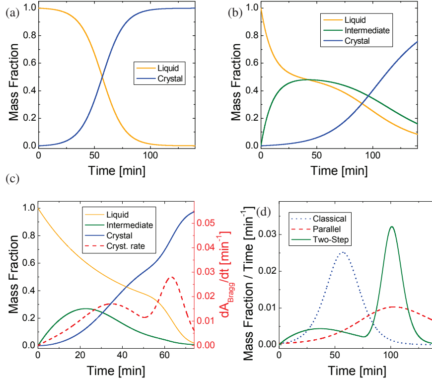
Figure 9 Comparison between different crystallization scenarios: (a) Classical nucleation from a homogeneous liquid and subsequent growth of the crystallites. (b) Parallel processes, representing the formation of an intermediate and the independent nucleation from the liquid with subsequent growth of the crystallites. (c) Two-step nucleation process involving the formation of an intermediate from which the crystals nucleate (see Table 1 for further details). The following parameter values were used to show the good qualitative agreement of the model with the data set in Figure 8a: k_e = 0.15 \text{ min}^{-1} , L_0 = 0.2 , \alpha_I = 0.2 , k_{gL} = 0.6 \text{ min}^{-1} , k_I = 0.03 \text{ min}^{-1} , k_n = 0.02 \text{ min}^{-1} , k_{gI} = 0.2 \text{ min}^{-1} . An additional model plot reproducing the data set in Figure 8b can be found in the S.I., Figure S3). (d) Comparison of the crystallization rates dC/dt . While one-step and parallel nucleation processes show a monotonous speed-up until saturation, the two-step process can have a non-monotonous signature with two maxima. The model parameters were chosen for all three models to be the same: k_I = 0.05 \text{ min}^{-1} , k_n = 0.02 \text{ min}^{-1} , k_{gI} = 0.1 \text{ min}^{-1} , k_{gL} = 0.2 \text{ min}^{-1} , k_e = 1.0 \text{ min}^{-1} , L_0 = 0.7 , \alpha_I = 0.2 .
