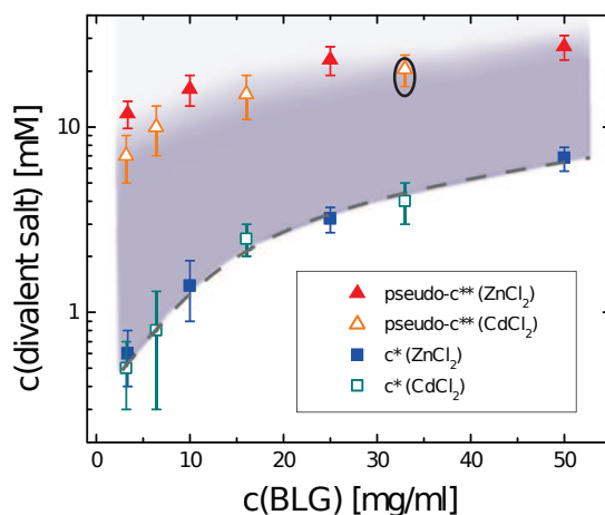
Figure 2 Experimental phase diagram of BLG with \text{ZnCl}_2 and \text{CdCl}_2 31,47 . Both salts share the similar c^* , below and above which the protein solutions are clear and turbid, respectively. Further increasing salt concentration, samples become gradually less turbid, but not completely clear again, and this transition zone is denoted as pseudo – c^{**} . The black ellipse marks the conditions mainly used in this work (33 mg/ml BLG with 15-20 mM \text{CdCl}_2 ).
