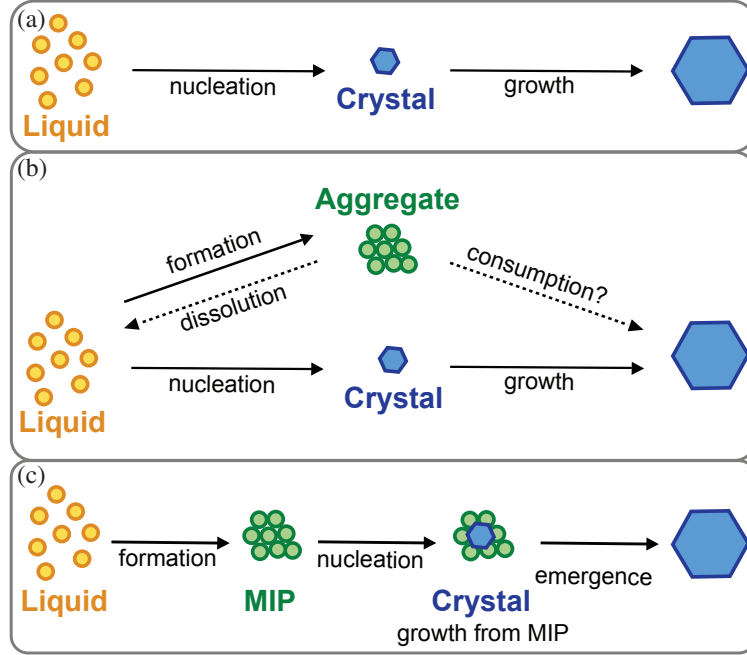
Figure 1 Illustrations of different pathways of crystal nucleation and growth. (a) Classical one-step pathway. (b) Parallel process of aggregate formation and crystal nucleation. (c) Multi-step process with precursor (MIP) for nucleation.
