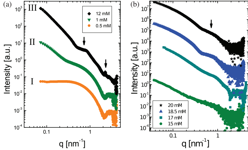
Figure 5 (a) SAXS measurements at a protein concentration of 6.5 mg/ml with CdCl 2 concentrations covering all three regimes of RC (marked by I, II, III). (b) Selected SAXS profiles at the time when the broad peak is well developed for samples in regime III with 33 mg/ml BLG and 15, 17, 18.5 and 20 mM CdCl 2 , respectively. Data are shifted upward for clarity.
