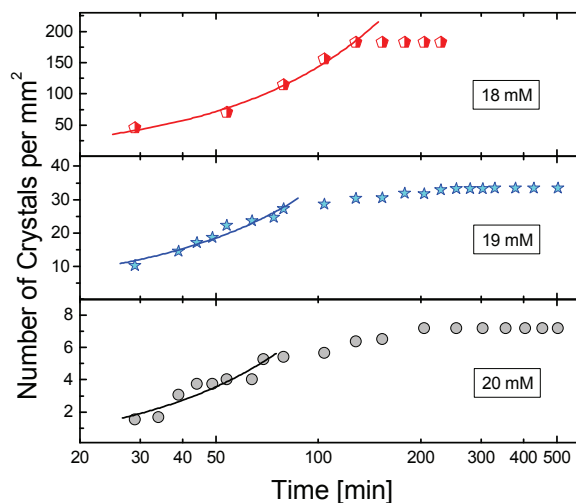
Figure 4 Number of crystals as a function of time in a normalized area from Figure 3 for samples with 18 mM, 19 mM and 20 mM \text{CdCl}_2 . For the 19 and 20 mM plots, three series of picture sets were analyzed and averaged for better statistics.
