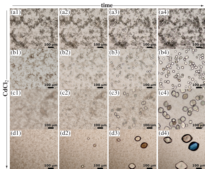
Figure 3 Image series of protein crystallization for samples with a BLG concentration of 33 mg/ml and \text{CdCl}_2 at different time: (a) 17 mM, (b) 18 mM, (c) 19 mM and (d) 20 mM (increasingly less turbid). (a1) 0, (a2) 50 min (a3) 75 min (a4) 100 min after preparation. (b1) 0 (b2) 75 min (b3) 100 min (b4) 3 h. (c1) 0, (c2) 100 min, (c3) 3 h, (c4) 6 h. (d1) 0, (d2) 3 h, (d3) 6 h and (d4) 10 h. Videos of the crystallization process in (a) and (d) can be found in online supporting materials.
