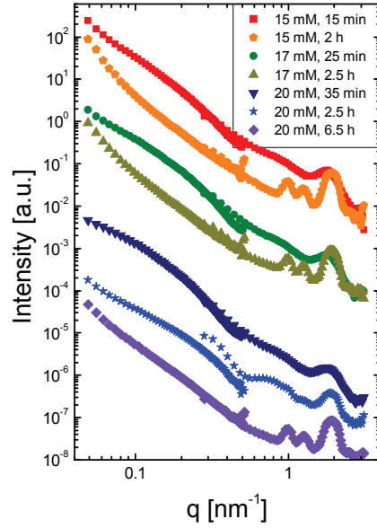
Figure 6 BLG 33 mg/ml with 15, 17 and 20 mM \text{CdCl}_2 in \text{D}_2\text{O} measured by SANS. Data are shifted upward for clarity. The mismatch of the SANS curves (especially visible for 20 mM after 2.5 h) was caused by measurements at different detector positions together with the fast kinetics occurring in the sample.
